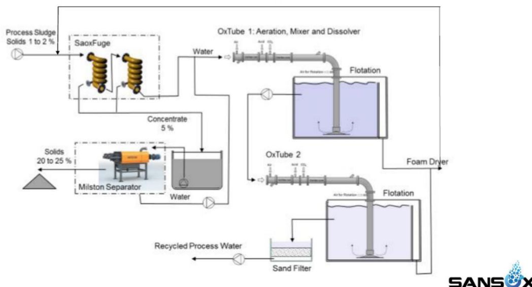
Figure 5. Overall VOxSton system and VOxFlotation system (right-hand-side part) (SansOx Brochure, 2016)
